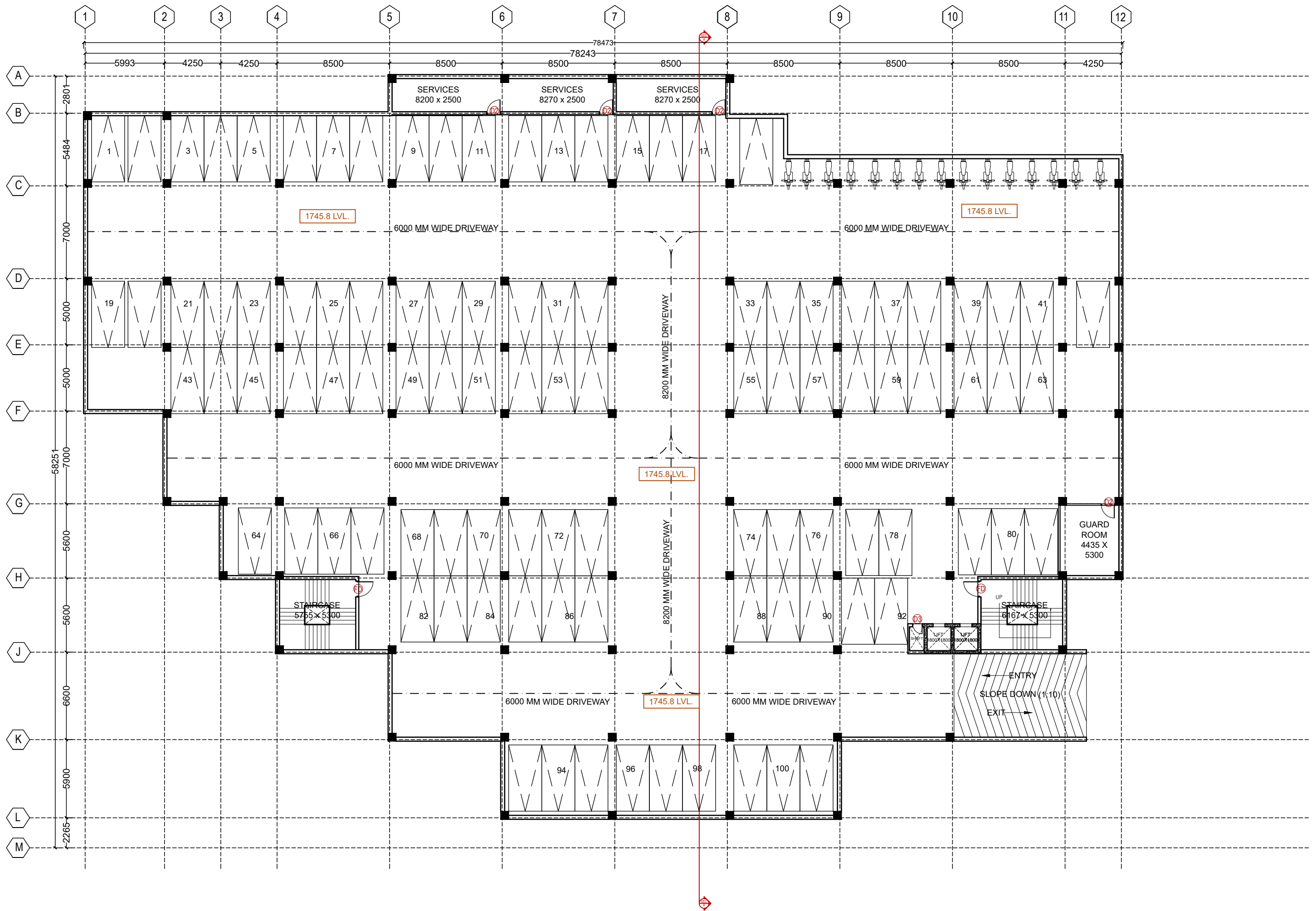
BASEMENT PARKING PLAN(LVL. 1745.8)
