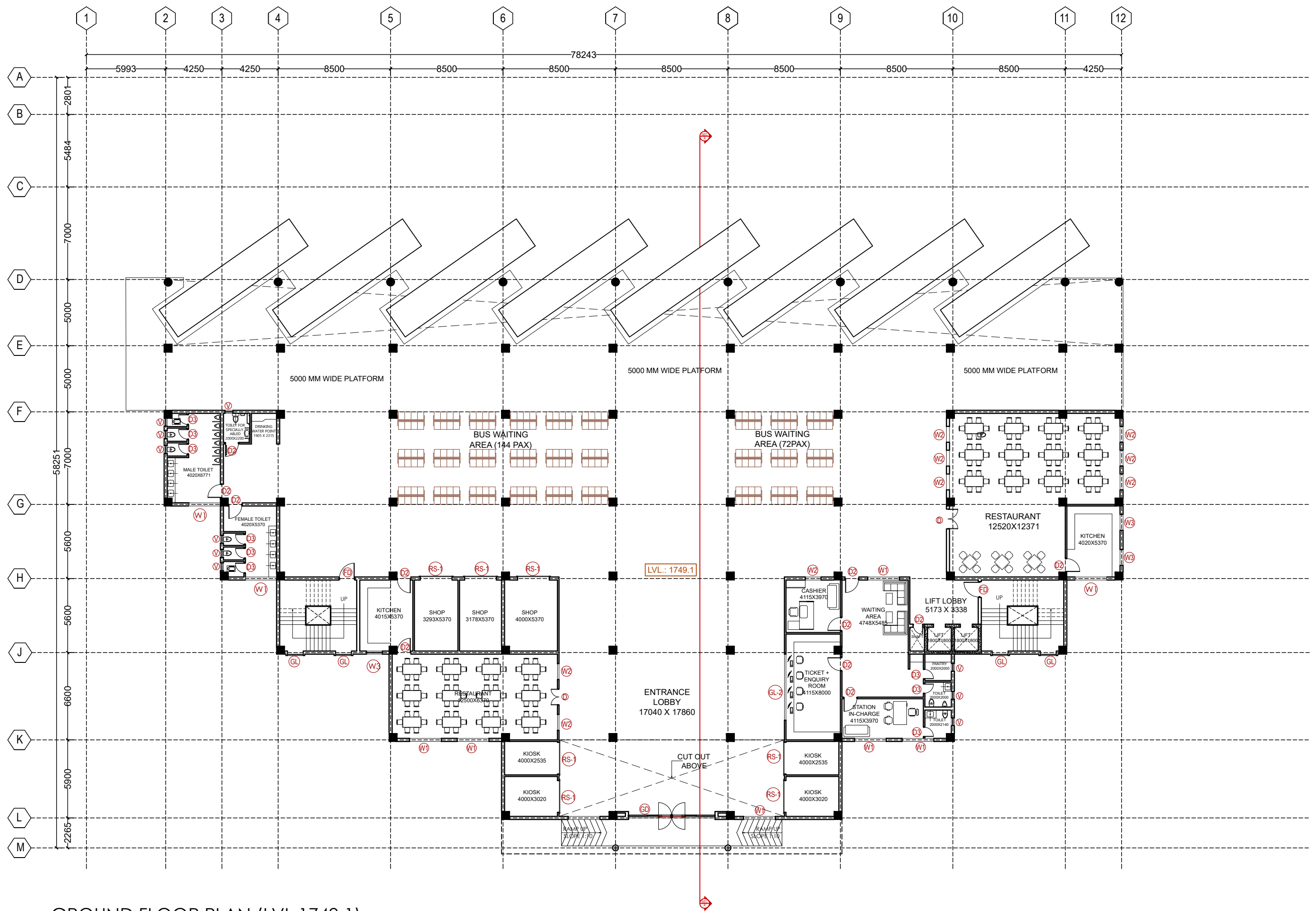
GROUND FLOOR PLAN (LVL.1749.1)
